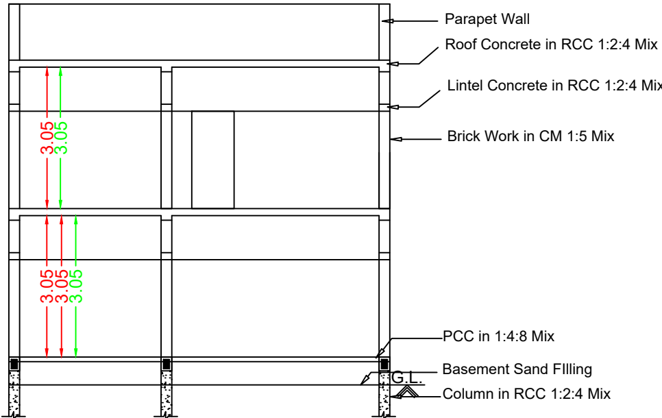
Section RR
