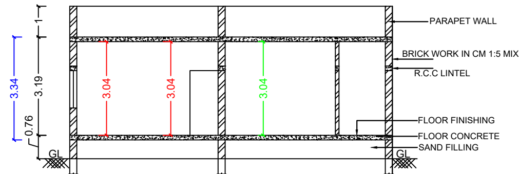
SECTION AT A1-A1
