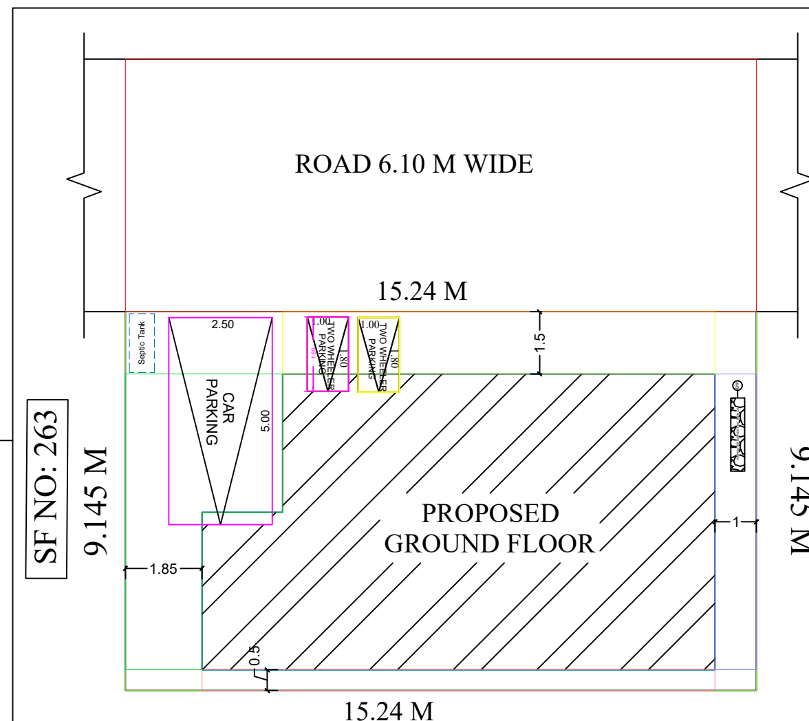
PLOT NO: G-14 SOUTH PART SITE PLAN (1:100)
