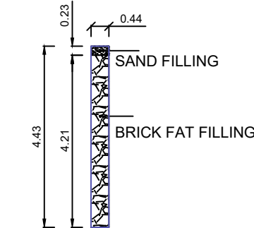
DETAILS OF PERCOLATION PIT
