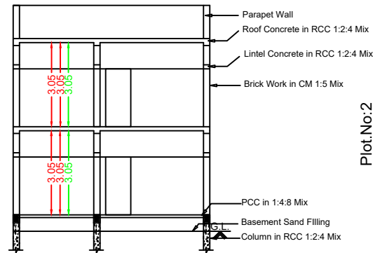
Section RR
