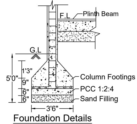
SECTION A1-A1
