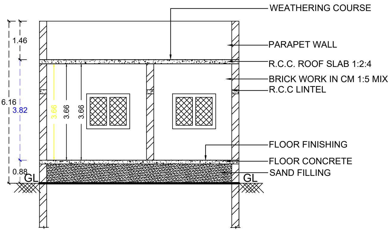
SECTION A1-A1
