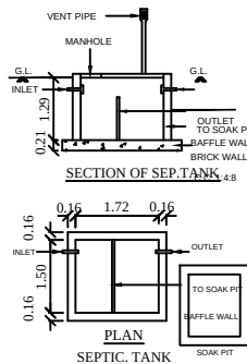
SECTION OF SEP. TANK
