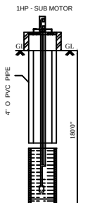
Bore Well Details
