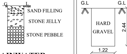
RAINWATER HARVESTING PIT
