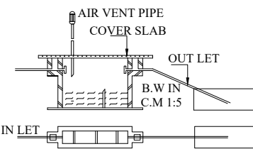
DETAILS OF SEPTIC TANK & D-TRENCH
