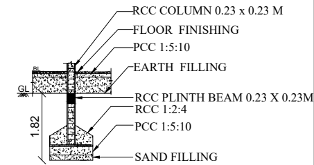
FOUNDATION DETAILS
