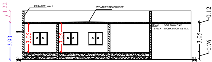
Section on-"AA"
