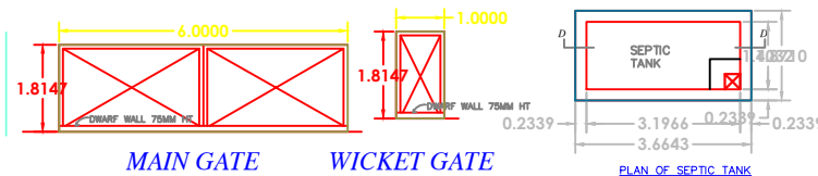
MAIN GATE
