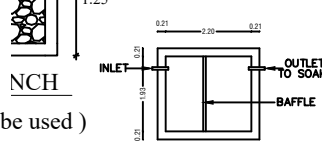
PLAN SEPTIC TANK
