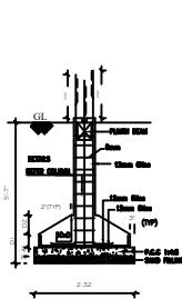
FOUNDATION DETAILS SCALE : 1:50.
