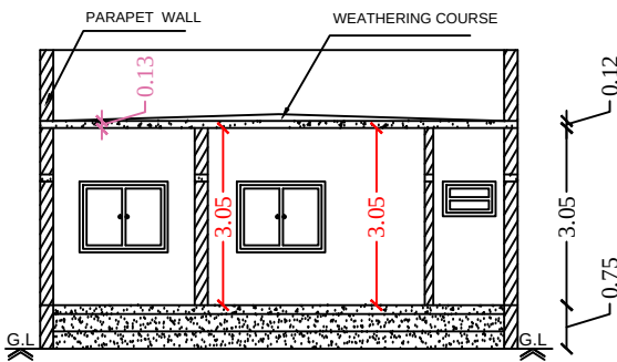
Section on-"AA"
