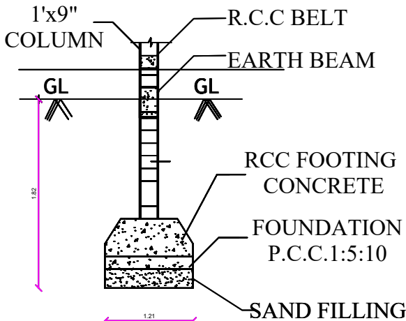
FOUNDATION DETAILS
