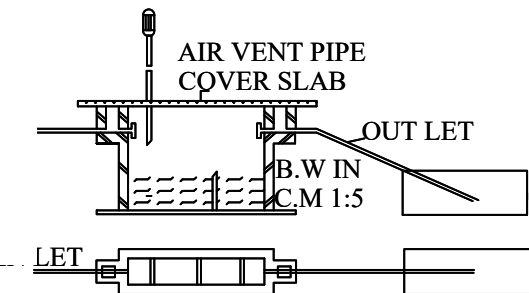
DETAILS OF SEPTIC TANK & D-TRENCH
