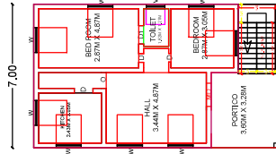
PRO. GROUND FLOOR PLAN
