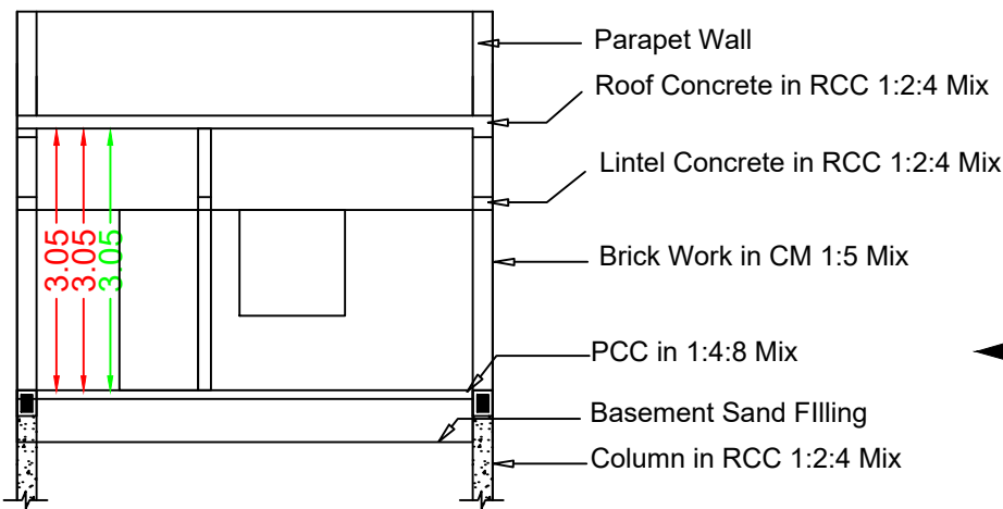
Section RR
