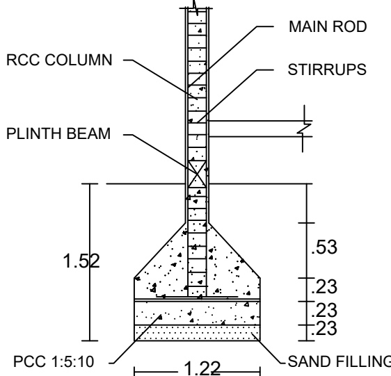
COLUMN DETAILS
