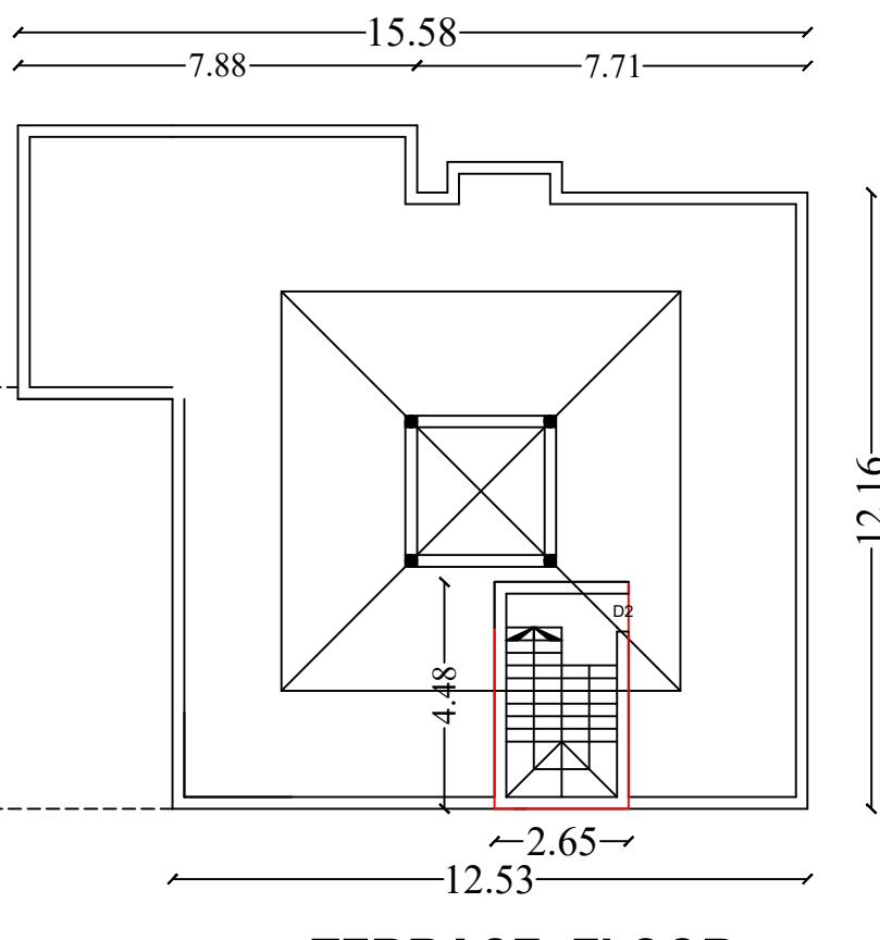
TERRACE FLOOR
