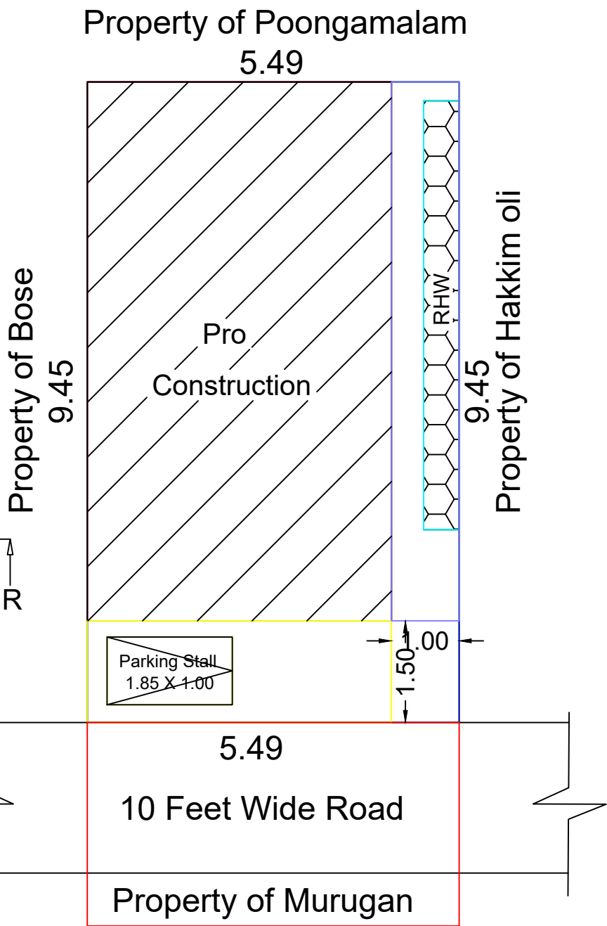
Site Plan
