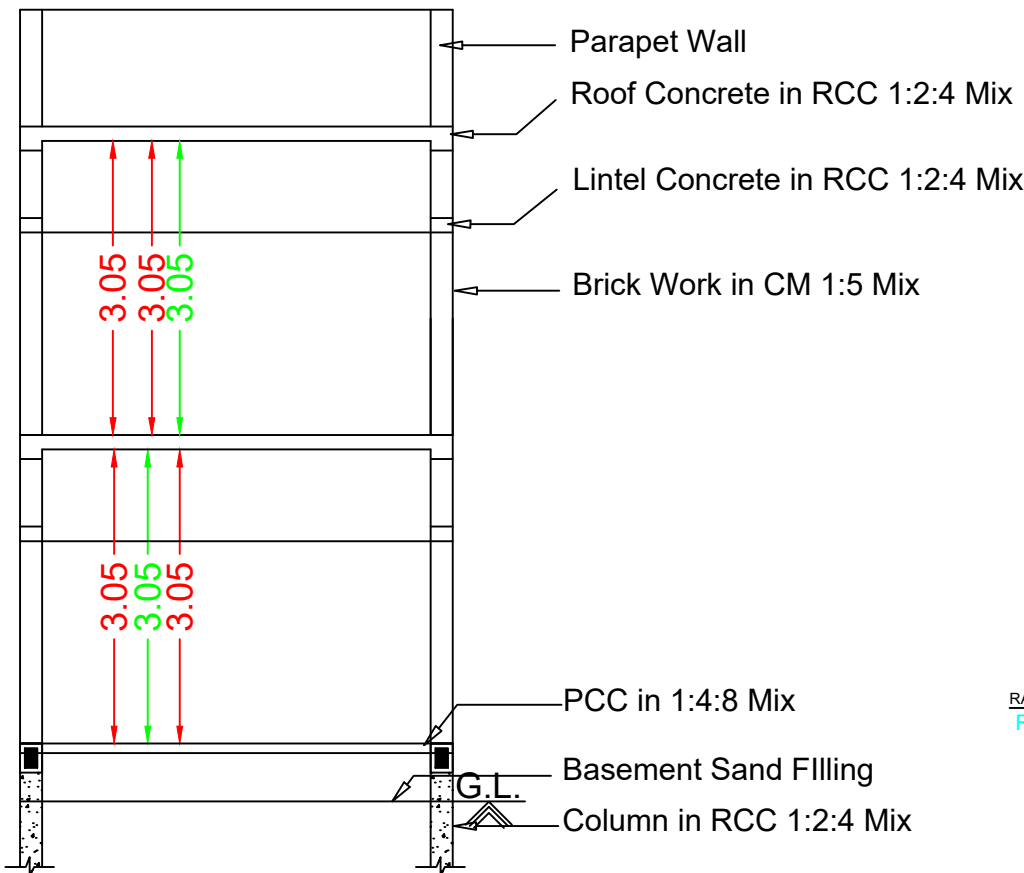
Section RR
