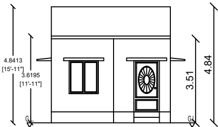
ELEVATION ON EAST
