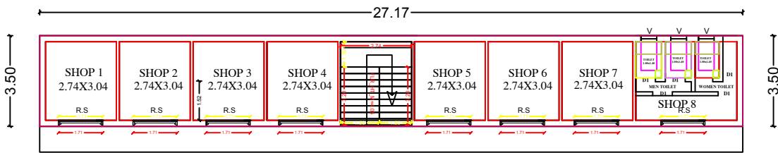
PRO.GROUND FLOOR PLAN
