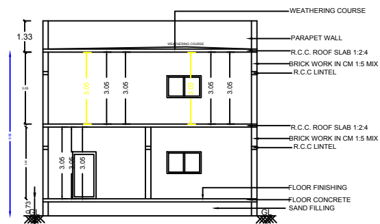
SECTION A1-A1
