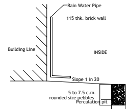
PERCOLATION PIT
