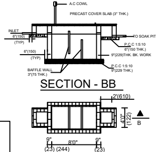
SEPTIC TANK:
