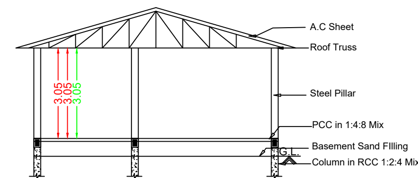
Section RR
