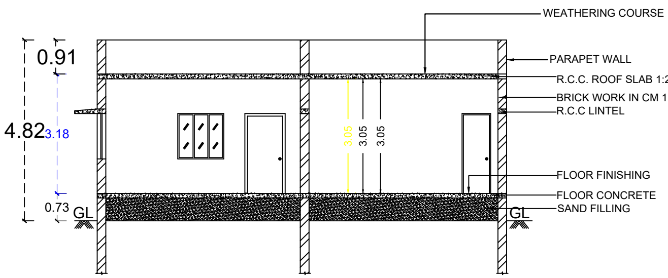
SECTION A1-A1
