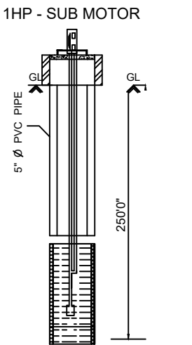
BOREWELL DETAILS
