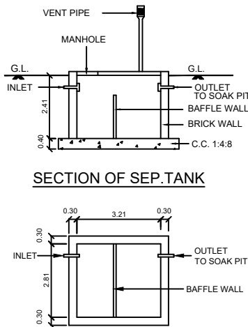
SEPTIC. TANK
