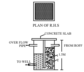
SECTIONS OF R.H.S.
