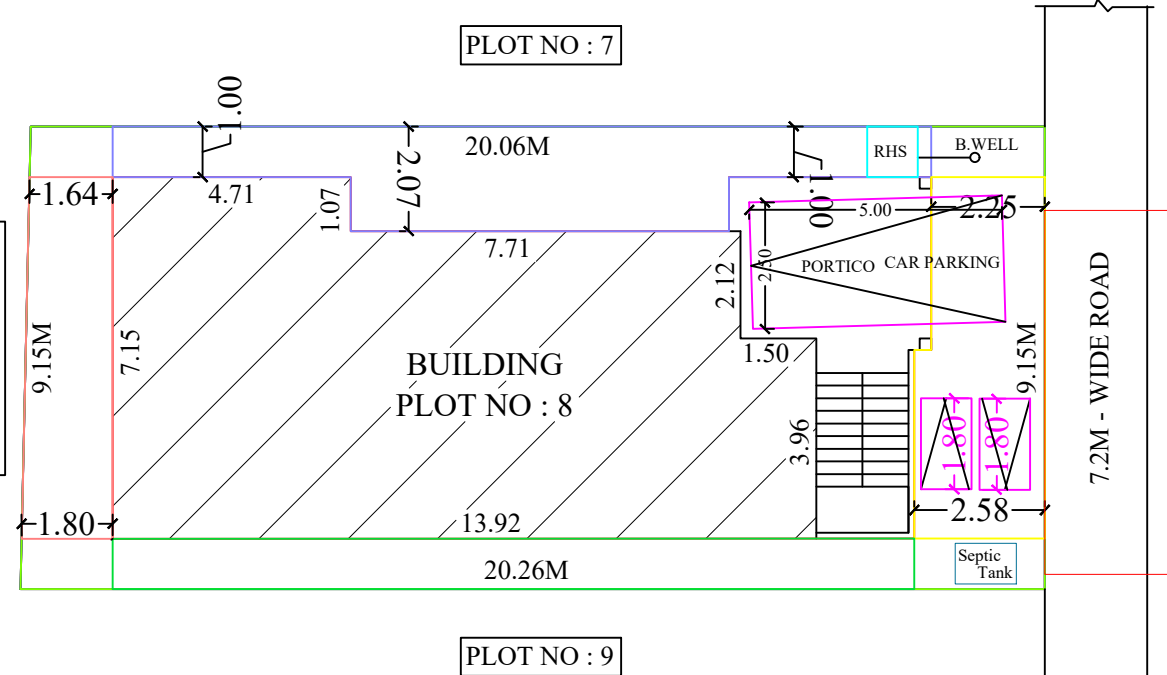
SITE PLAN (1:100)
