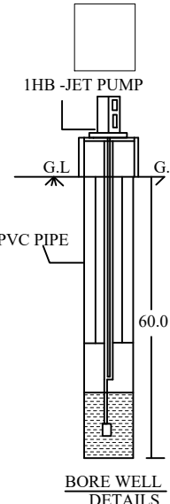
BORE WELL DETAILS
