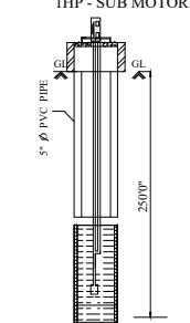
BOREWELL DETAILS
