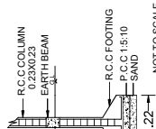
EXI. FOUNDATION DETAILS
