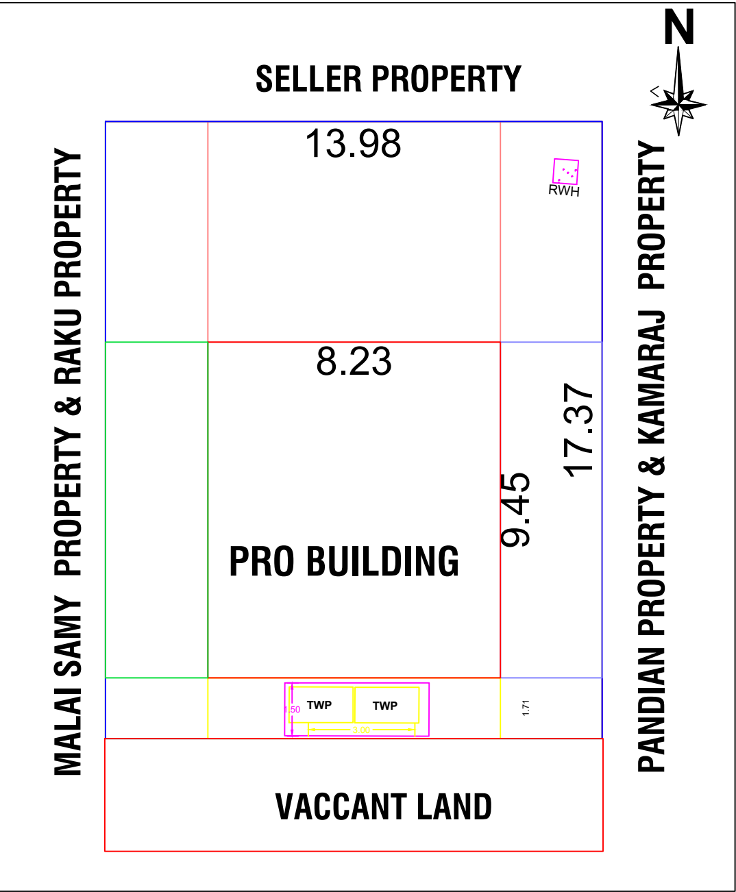
SITE PLAN
