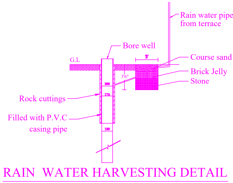
RAIN WATER HARVESTING DETAIL
