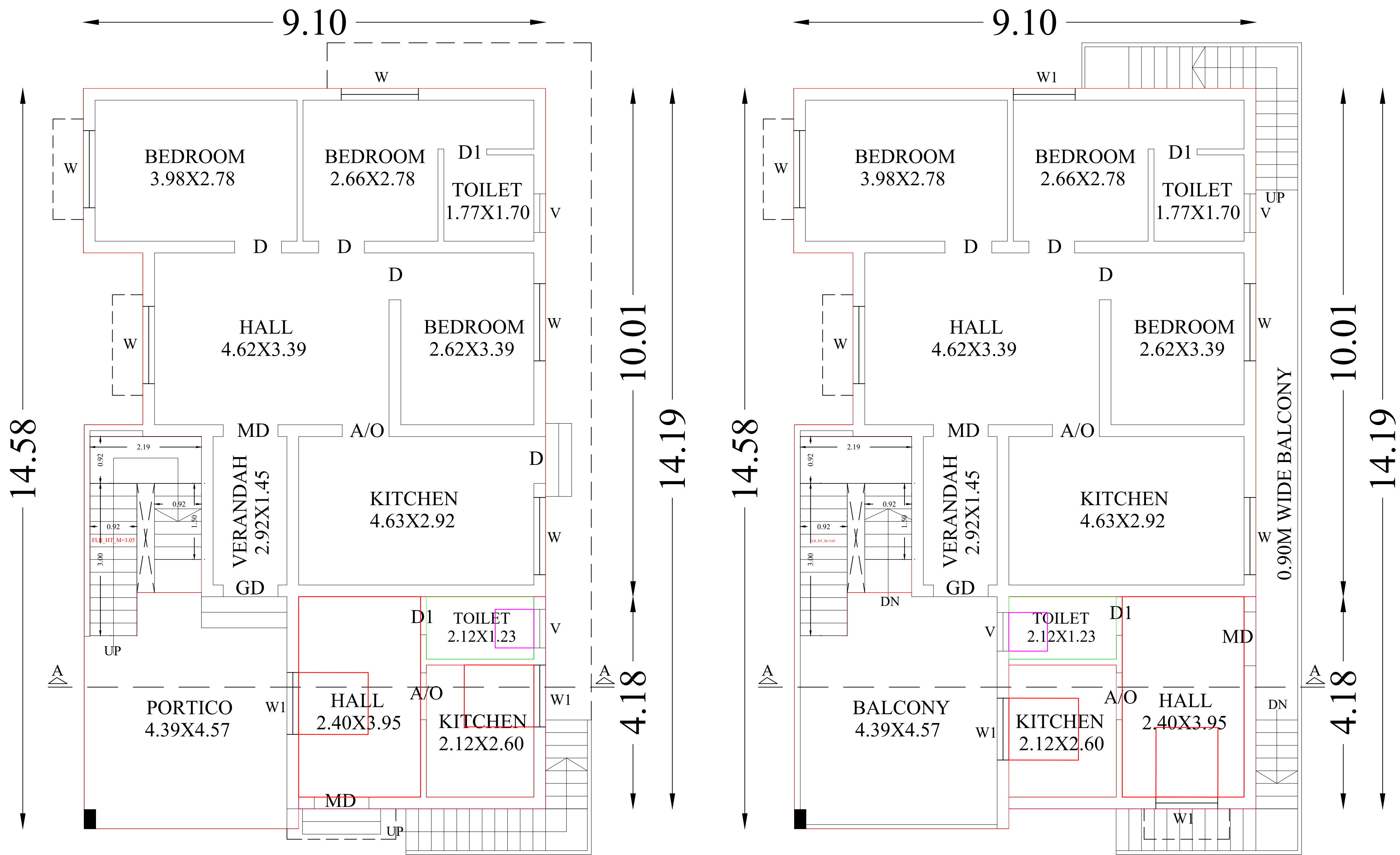
EXISTING & PROPOSED GROUND FLOOR PLAN
