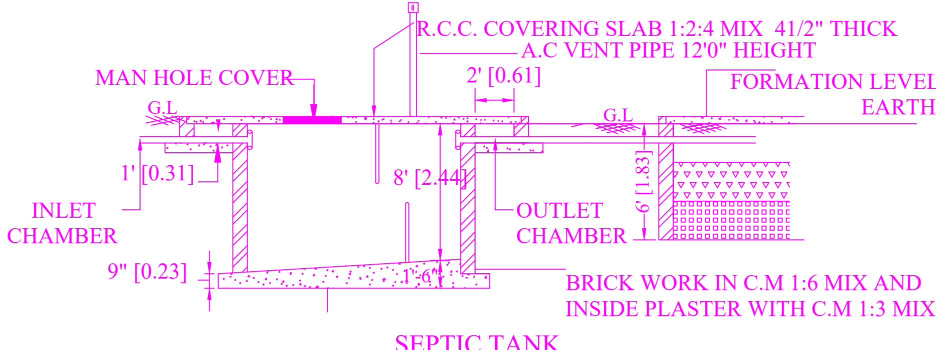
SEPTIC TANK
