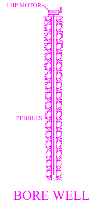
BORE WELL
