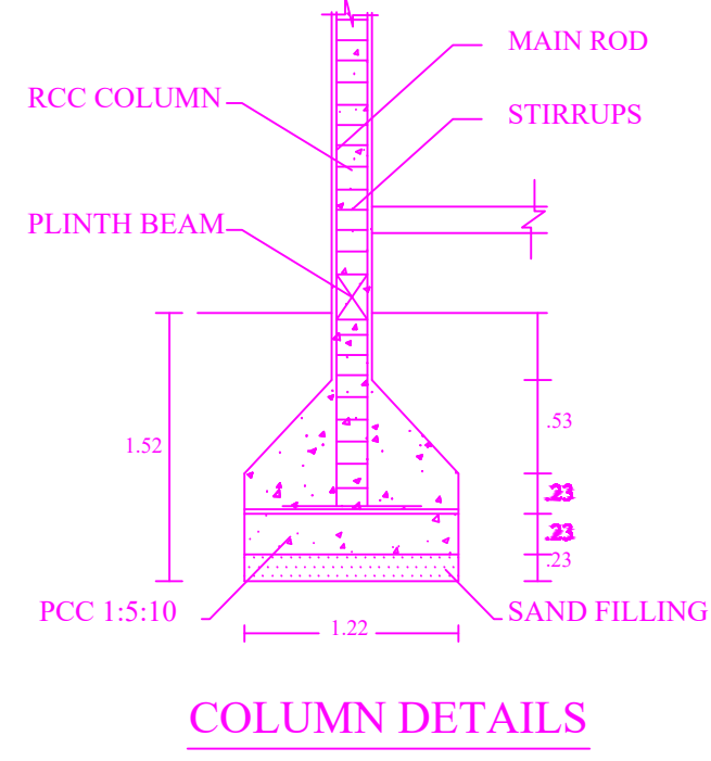
COLUMN DETAILS
