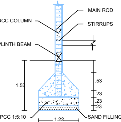
COLUMN DETAILS
