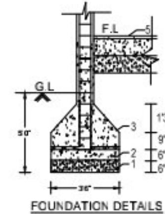
FOUNDATION DETAILS
