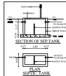
SECTION OF SEPTIC TANK
