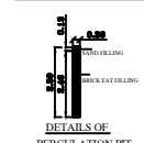
DETAILS OF PERCOLATION PIT
