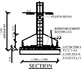
SECTION
