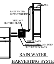
RAIN WATER HARVESTING SYSTEM
