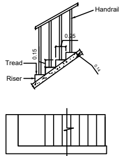
STAIRCASE DETAIL
