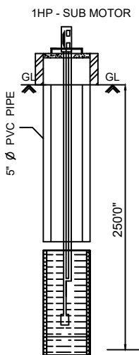
BOREWELL DETAILS
