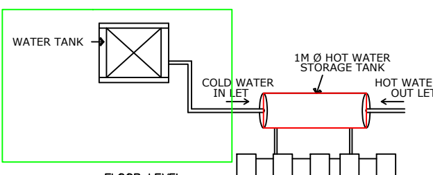
Solar Hot Water System Detail
