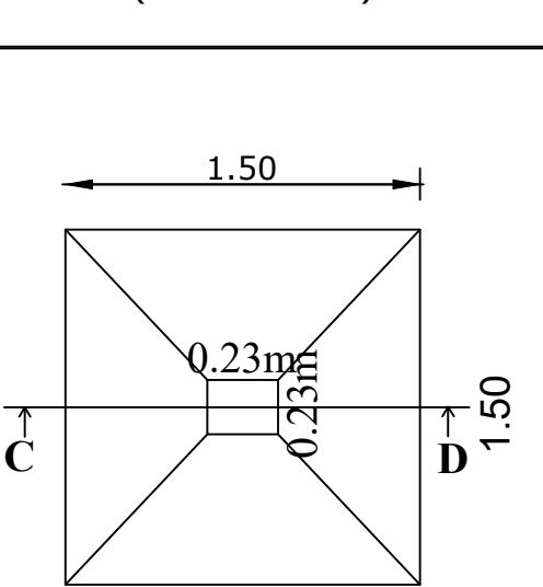
SECTION - 'CD'
