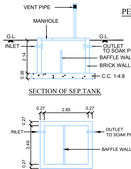
PLAN SEPTIC. TANK
