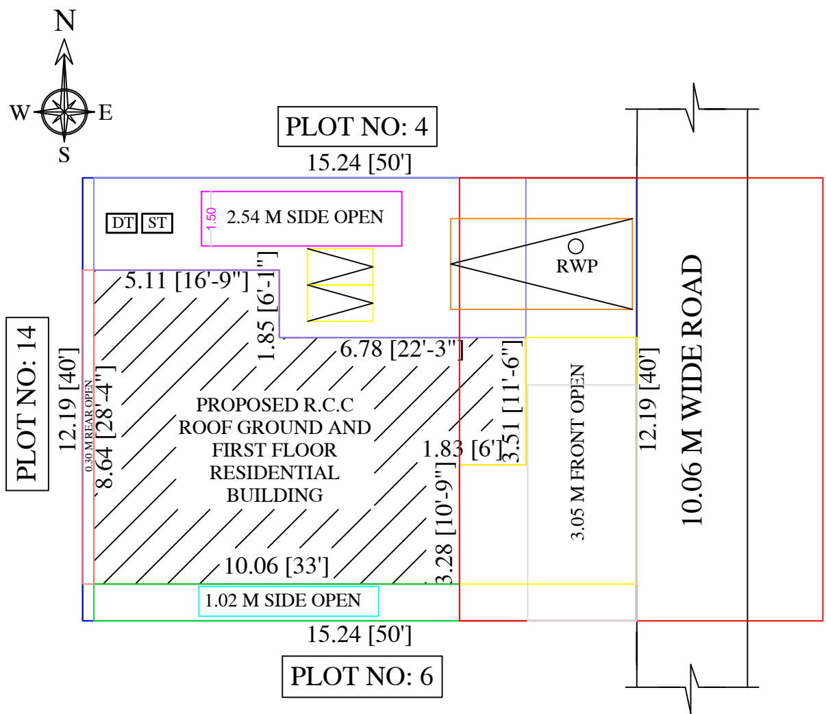
SITE PLAN
