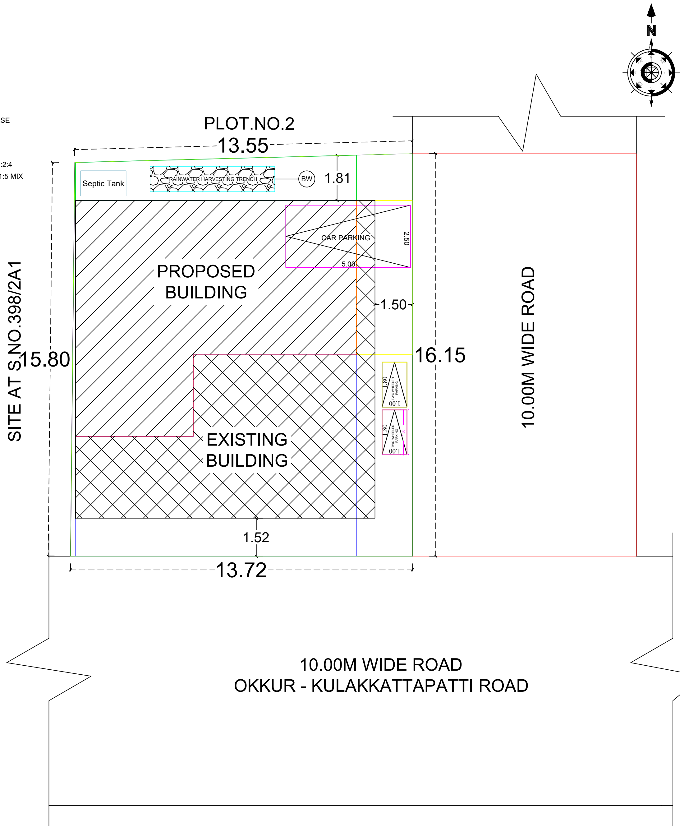
SITE PLAN (1:100)
