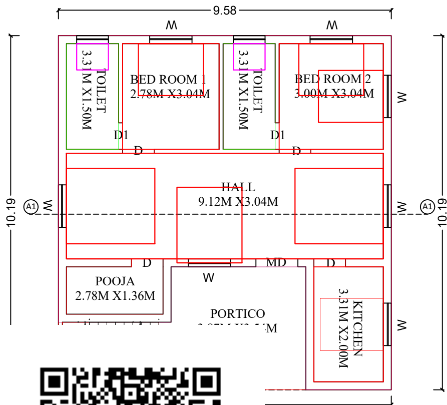
FLOOR PLAN
