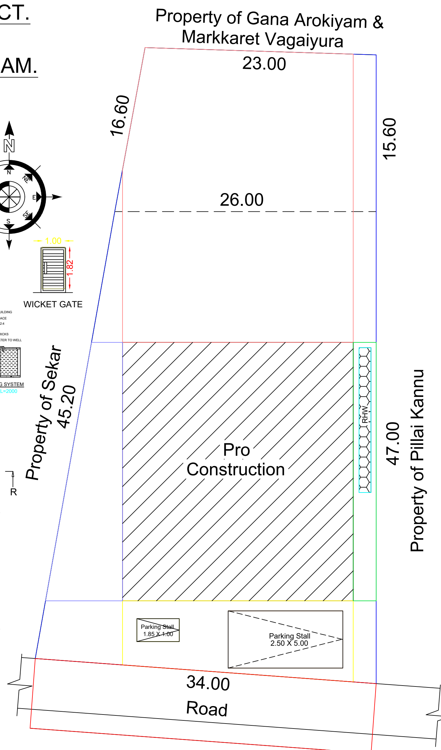
Site Plan(NTS)
