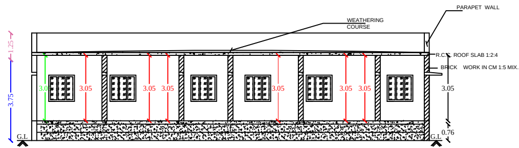
Section on-"AA"
