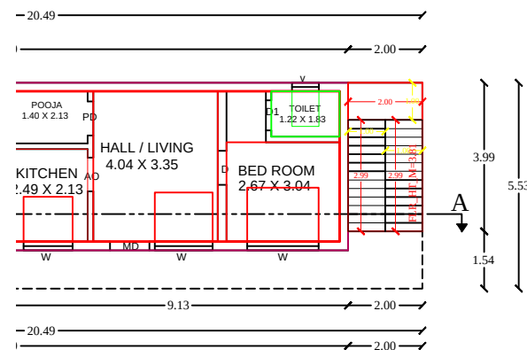
Floor - Ground
