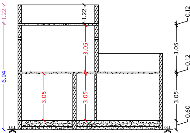
Section on-"AA"
