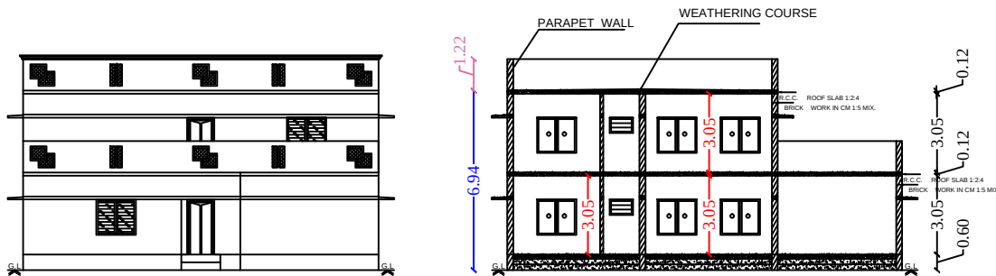
Front Elevation
