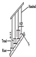
STAIRCASE DETAIL
