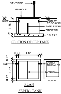
SEPTIC TANK
