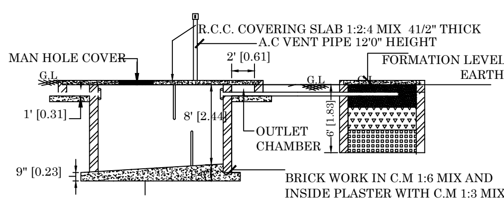
SEPTIC TANK
