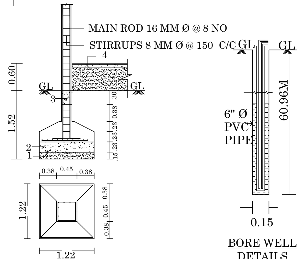
RCP COLUMN FOUNDATION DETAILS
