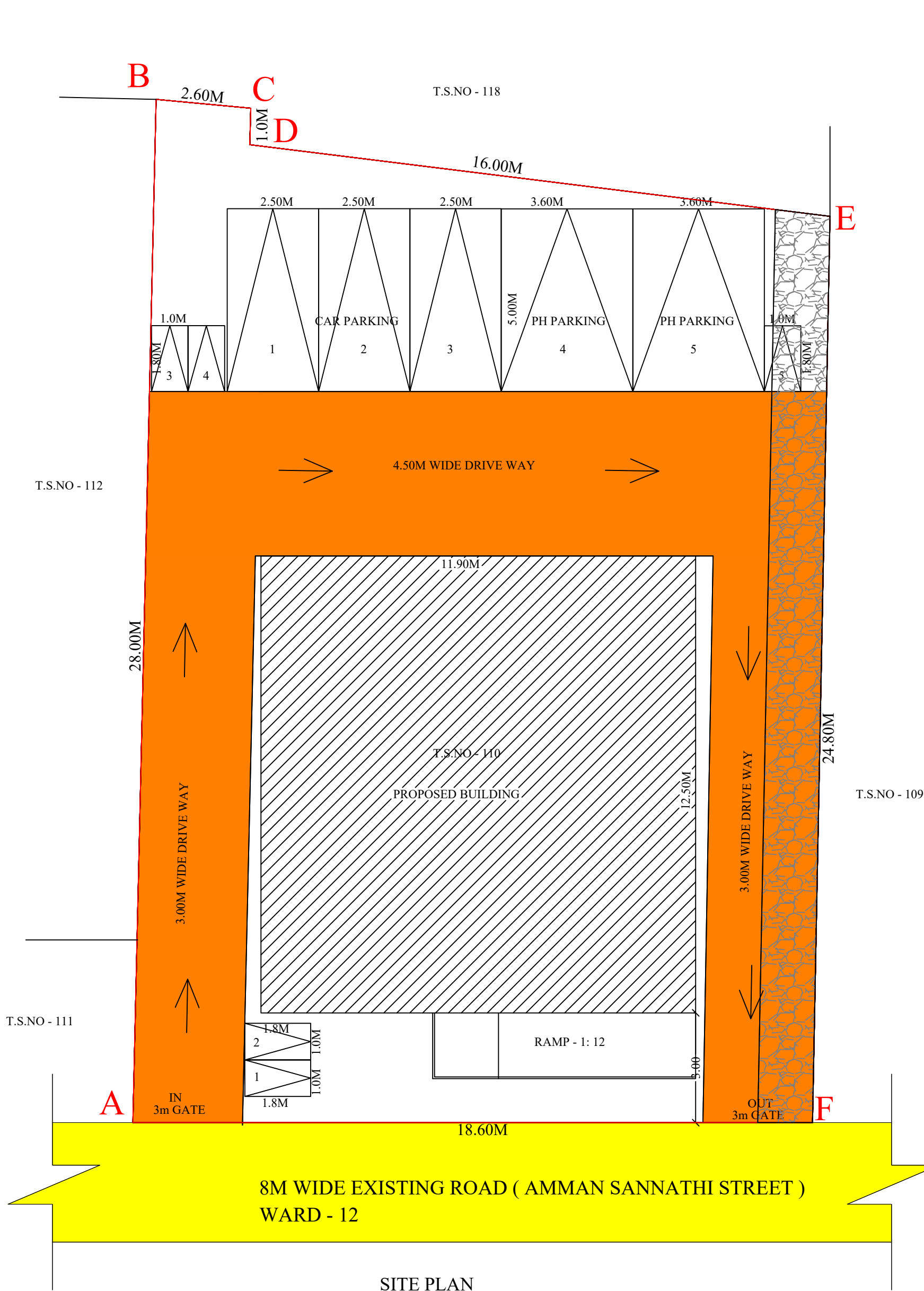
SITE PLAN
