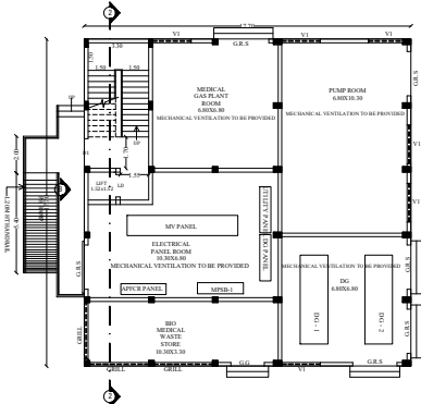
GROUND FLOOR PLAN (ADMIN BLOCK)
