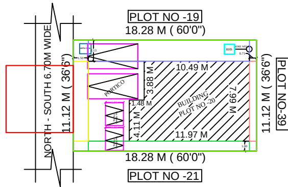
SITE PLAN (1:100)
