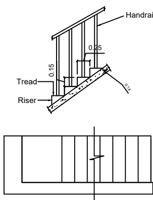
STAIRCASE DETAIL
