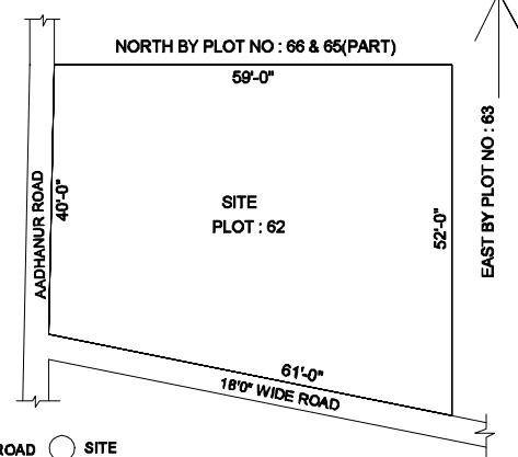
SITE LAYOUT
