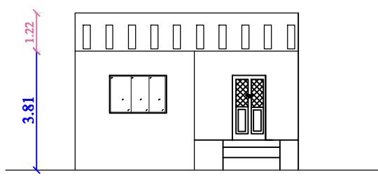
FRONT ELEVATION
