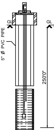
BOREWELL DETAILS
