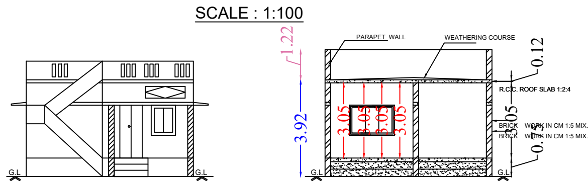
Section on-"AA"
